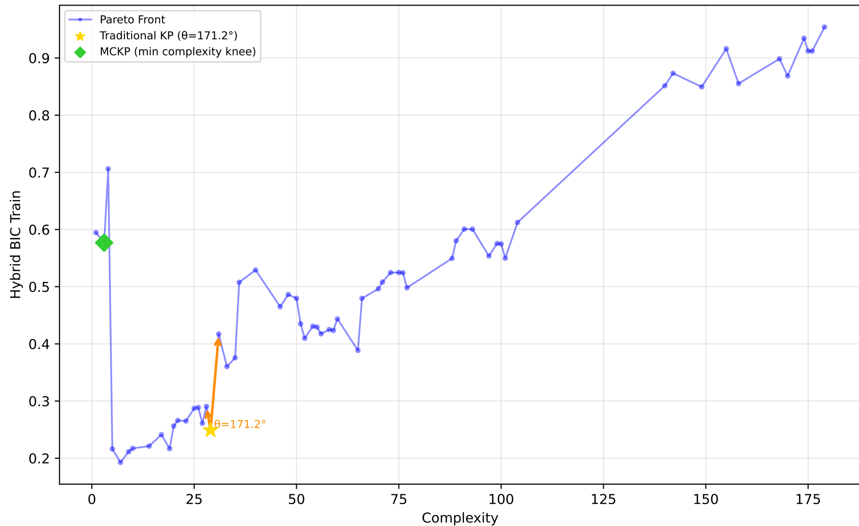
228_elusage - Run 16 - MVP - Hybrid BIC Train \lambda_1=0.00, \lambda_2=0.30, \lambda_3=0.00 | Difficulty: 0.72 | Method: hmr
