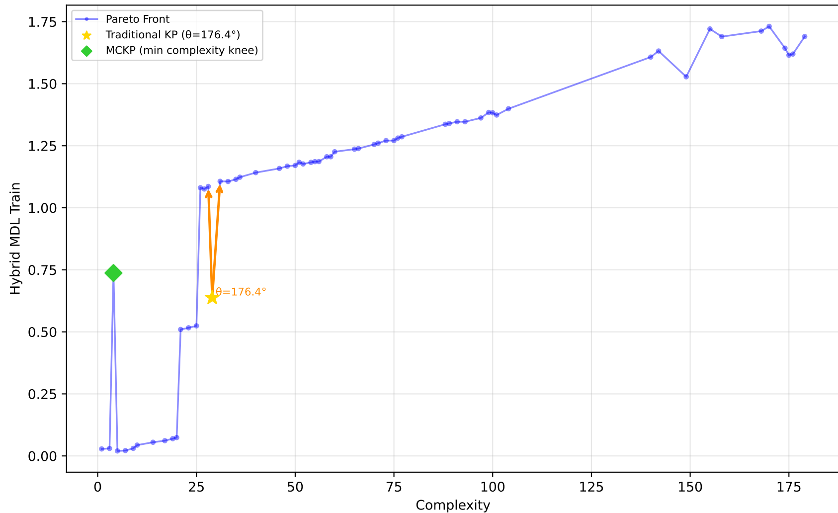
228_elusage - Run 16 - MVP - Hybrid MDL Train \lambda_1=0.00, \bar{\lambda}_2=0.00, \lambda_3=1.00 | Difficulty: 0.72 | Method: hmr
