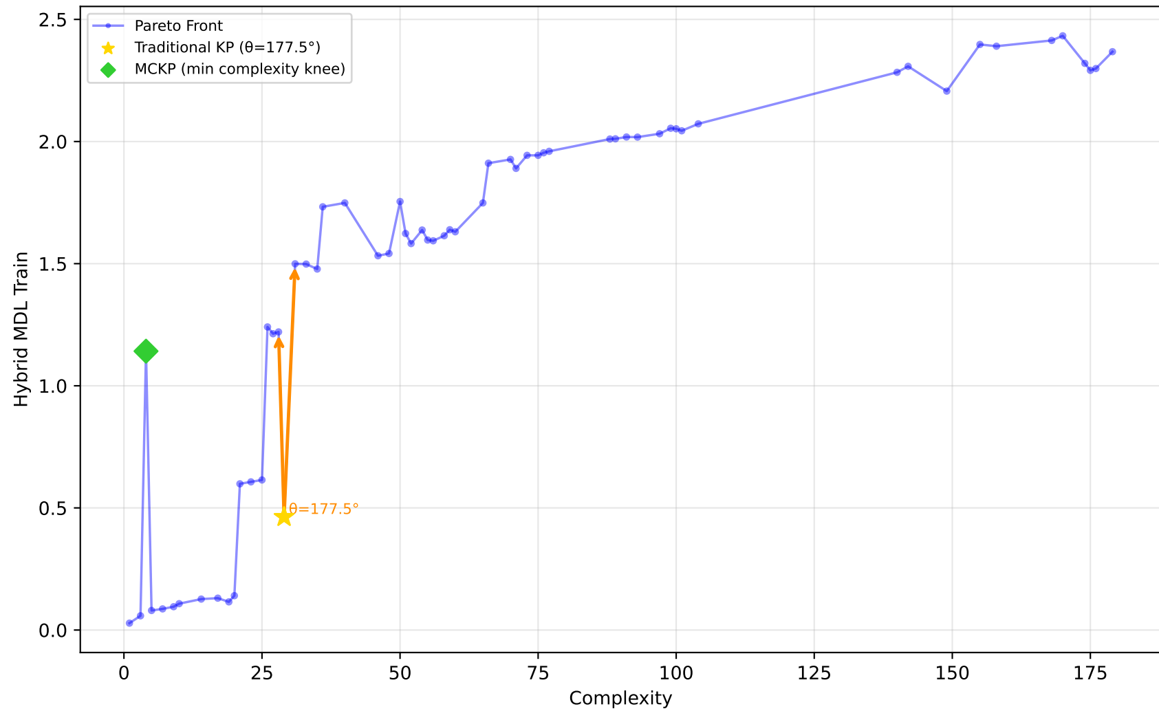
228_elusage - Run 16 - SVP - Hybrid MDL Train \lambda_1=0.60, \bar{\lambda}_2=0.60, \lambda_3=1.00 | Difficulty: 0.72 | Method: hmr
