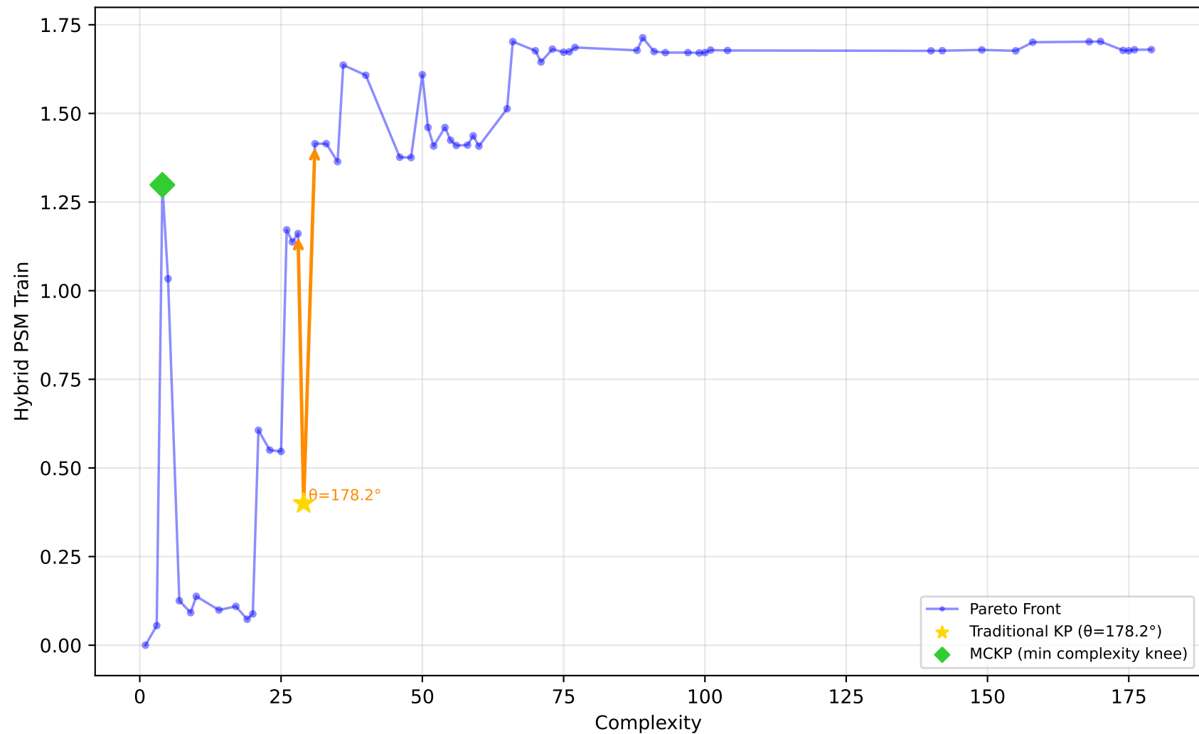
228_elusage - Run 16 - SVP - Hybrid PSM Train \lambda_1=0.60, \bar{\lambda}_2=0.60, \lambda_3=1.00 | Difficulty: 0.72 | Method: hmr
