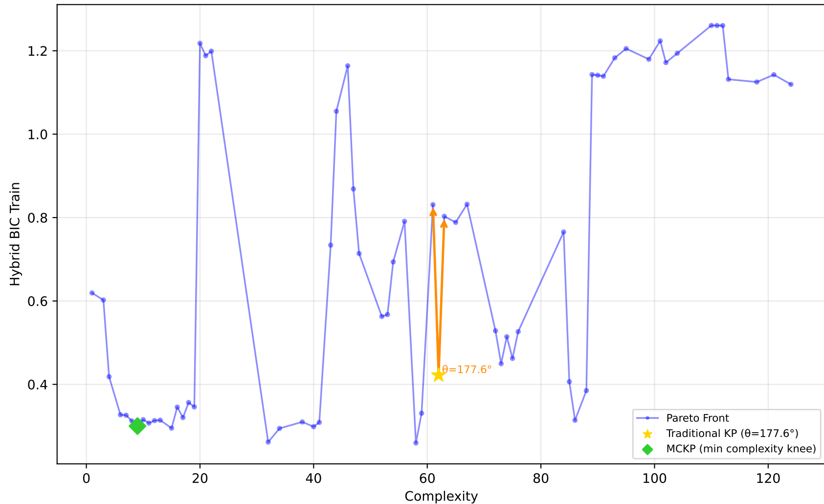
228_elusage - Run 17 - MVP - Hybrid BIC Train \lambda_1=0.00, \lambda_2=0.00, \lambda_3=1.00 | Difficulty: 0.69 | Method: hmr
