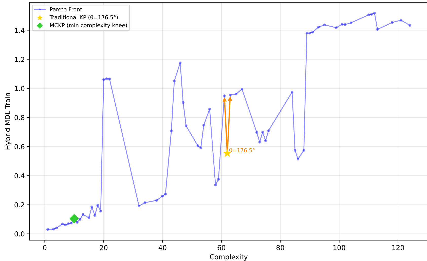
228_elusage - Run 17 - MVP - Hybrid MDL Train \lambda_1=0.00, \bar{\lambda}_2=0.00, \lambda_3=1.00 | Difficulty: 0.69 | Method: hmr
