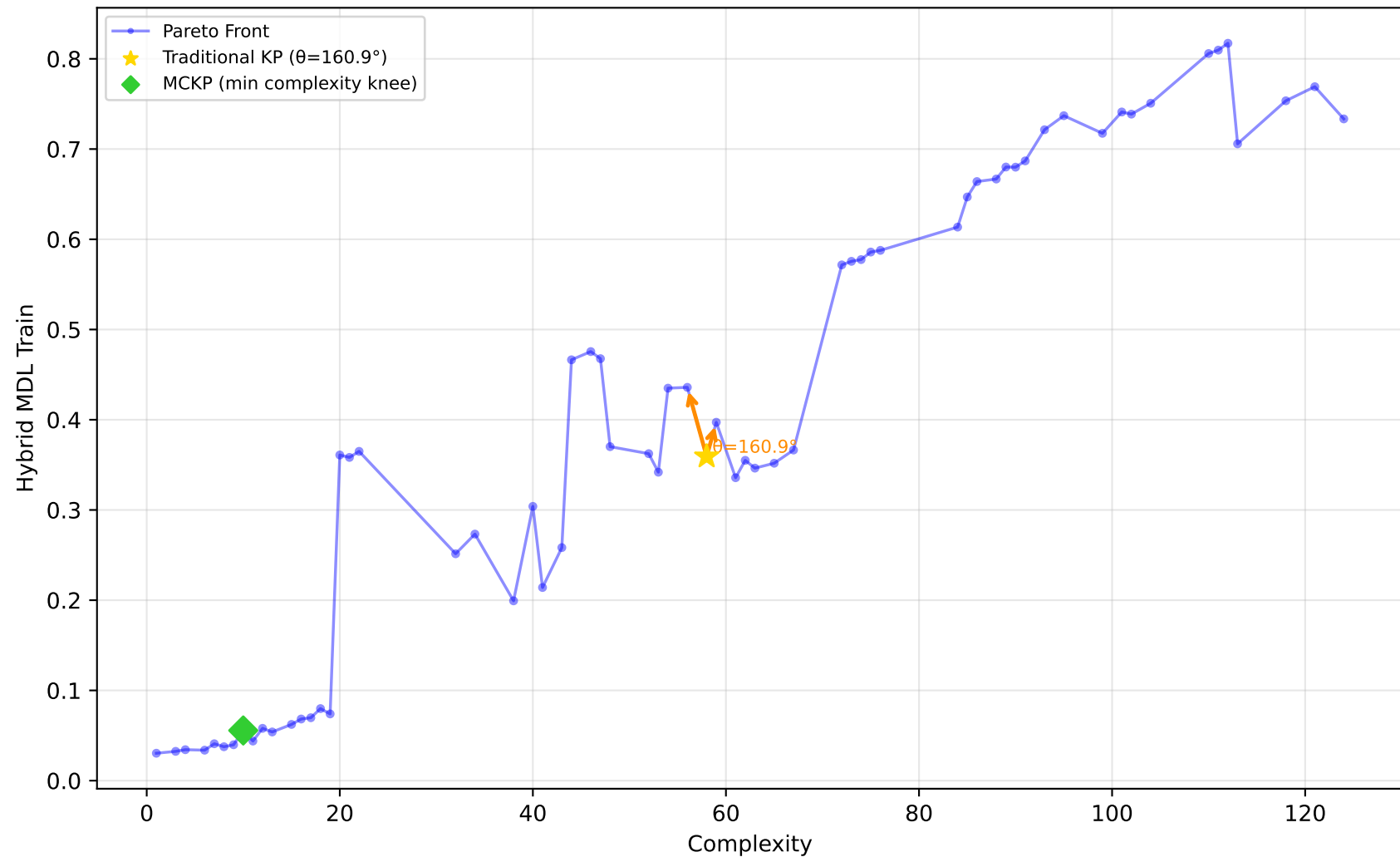
228_elusage - Run 17 - MVP - Hybrid MDL Train \lambda_1=0.00, \bar{\lambda}_2=0.30, \lambda_3=0.00 | Difficulty: 0.69 | Method: hmr
