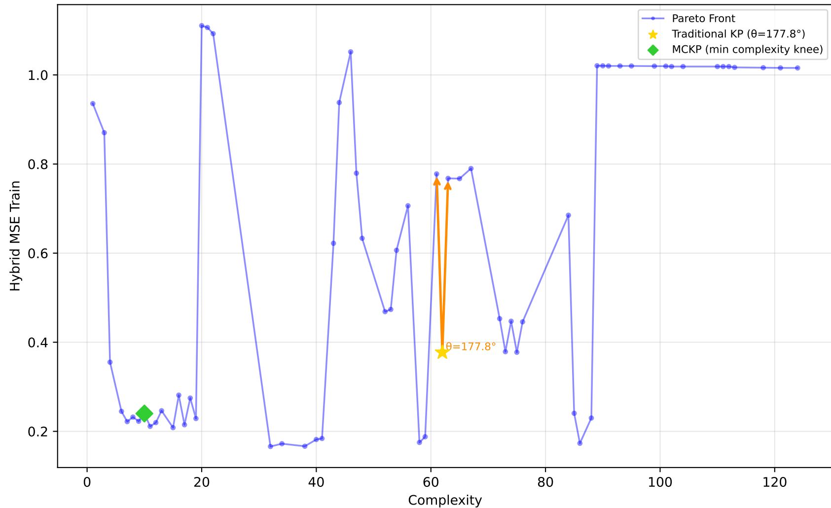
228 elusage - Run 17 - MVP - Hybrid MSE Train \lambda_1=0.00, \bar{\lambda}_2=0.00, \lambda_3=1.00 | Difficulty: 0.69 | Method: hmr
