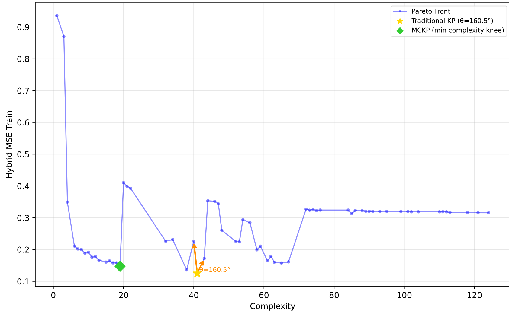
228_elusage - Run 17 - MVP - Hybrid MSE Train \lambda_1=0.00, \bar{\lambda}_2=0.30, \lambda_3=0.00 | Difficulty: 0.69 | Method: hmr
