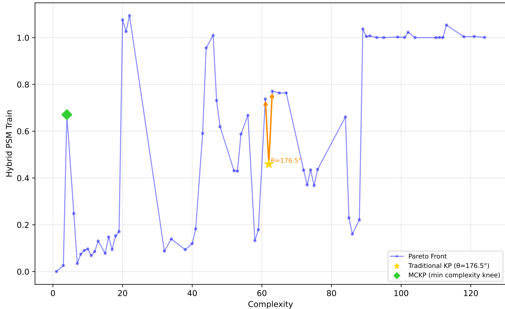
228_elusage - Run 17 - MVP - Hybrid PSM Train \lambda_1=0.00, \bar{\lambda}_2=0.00, \lambda_3=1.00 | Difficulty: 0.69 | Method: hmr
