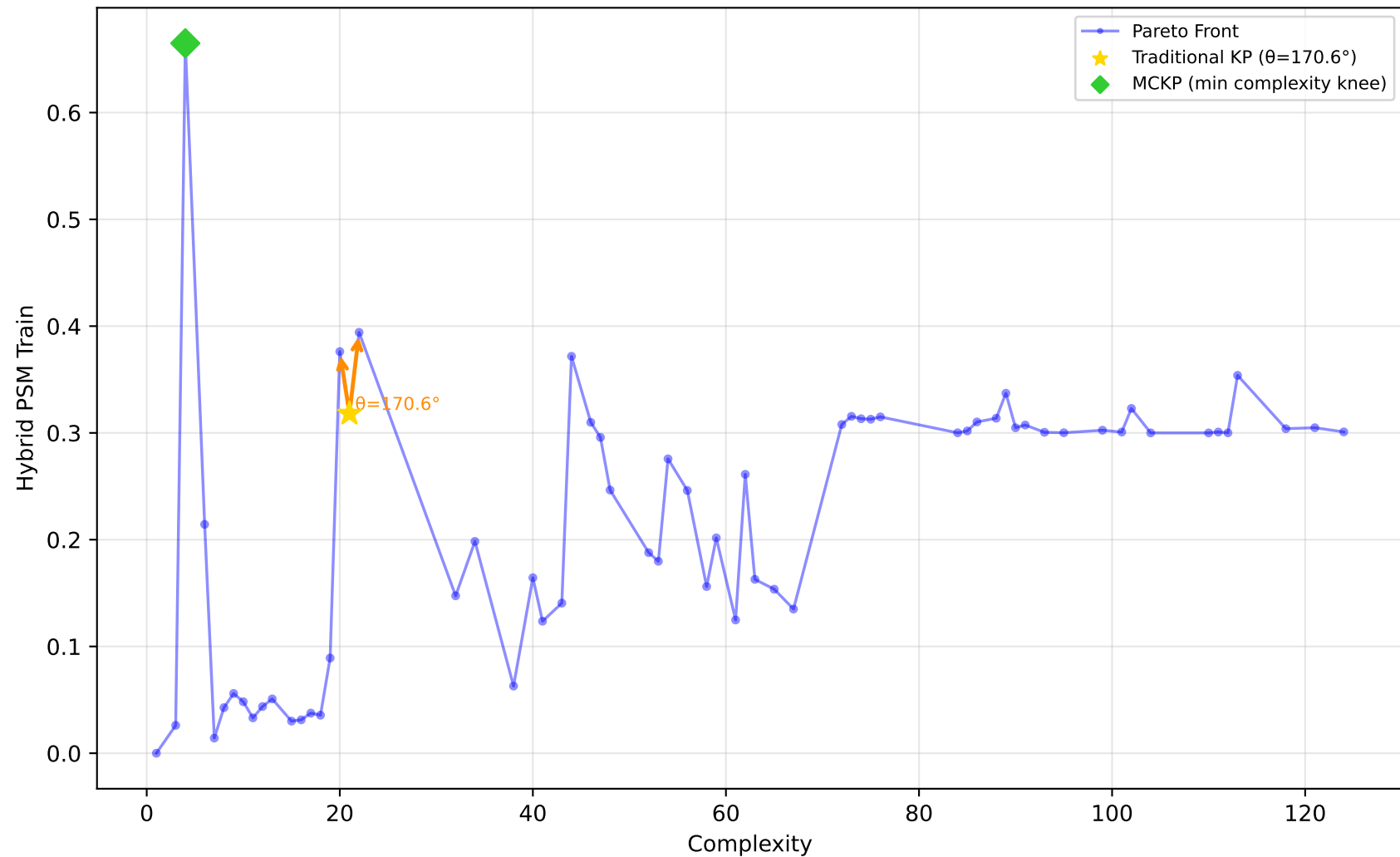
228_elusage - Run 17 - MVP - Hybrid PSM Train \lambda_1=0.00, \bar{\lambda}_2=0.30, \lambda_3=0.00 | Difficulty: 0.69 | Method: hmr
