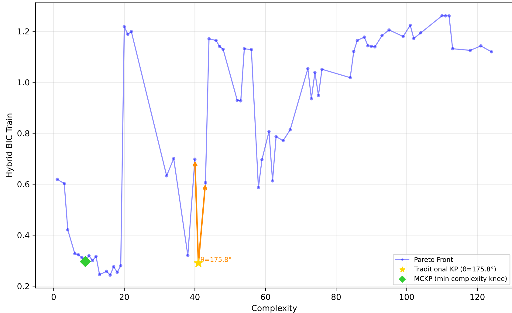
228_elusage - Run 17 - SVP - Hybrid BIC Train \lambda_1=0.00, \lambda_2=1.00, \lambda_3=0.00 | Difficulty: 0.69 | Method: hmr
