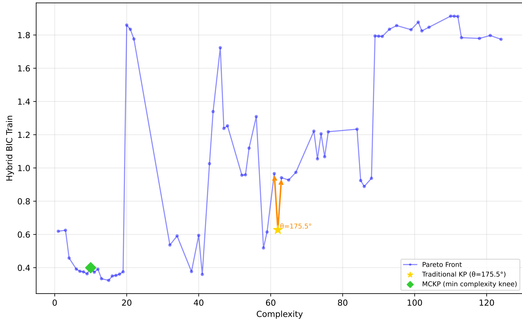
228_elusage - Run 17 - SVP - Hybrid BIC Train \lambda_1=0.60, \lambda_2=0.60, \lambda_3=1.00 | Difficulty: 0.69 | Method: hmr
