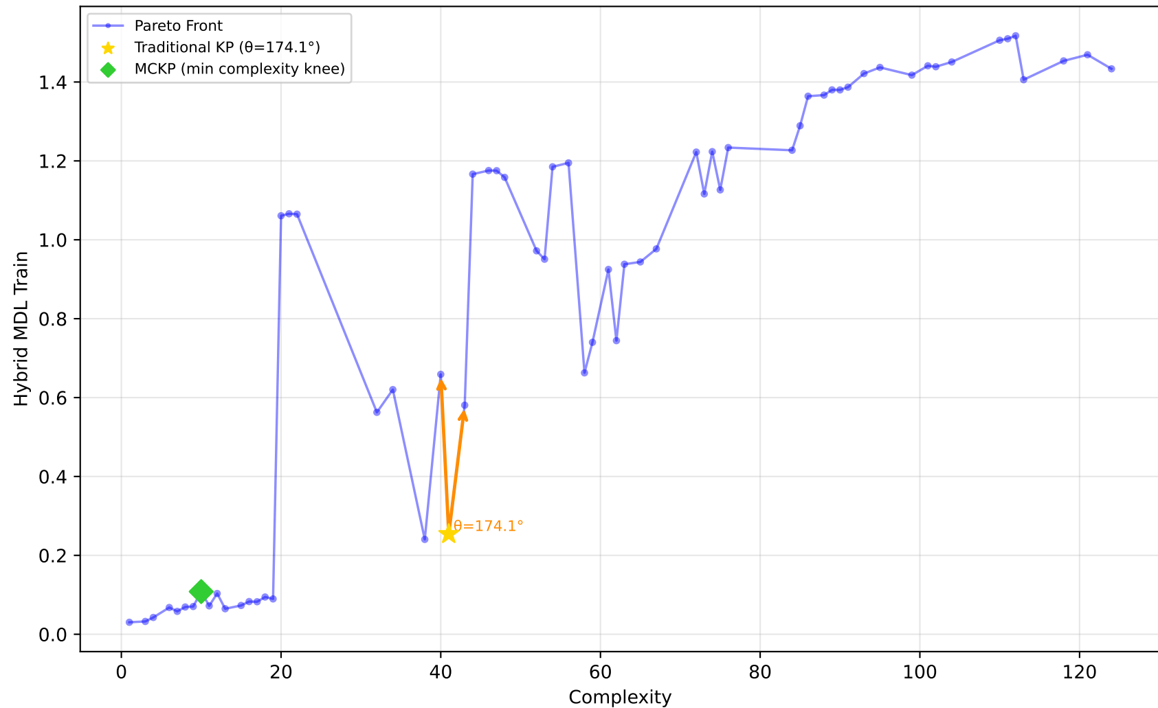
228_elusage - Run 17 - SVP - Hybrid MDL Train \lambda_1=0.00, \bar{\lambda}_2=1.00, \lambda_3=0.00 | Difficulty: 0.69 | Method: hmr
