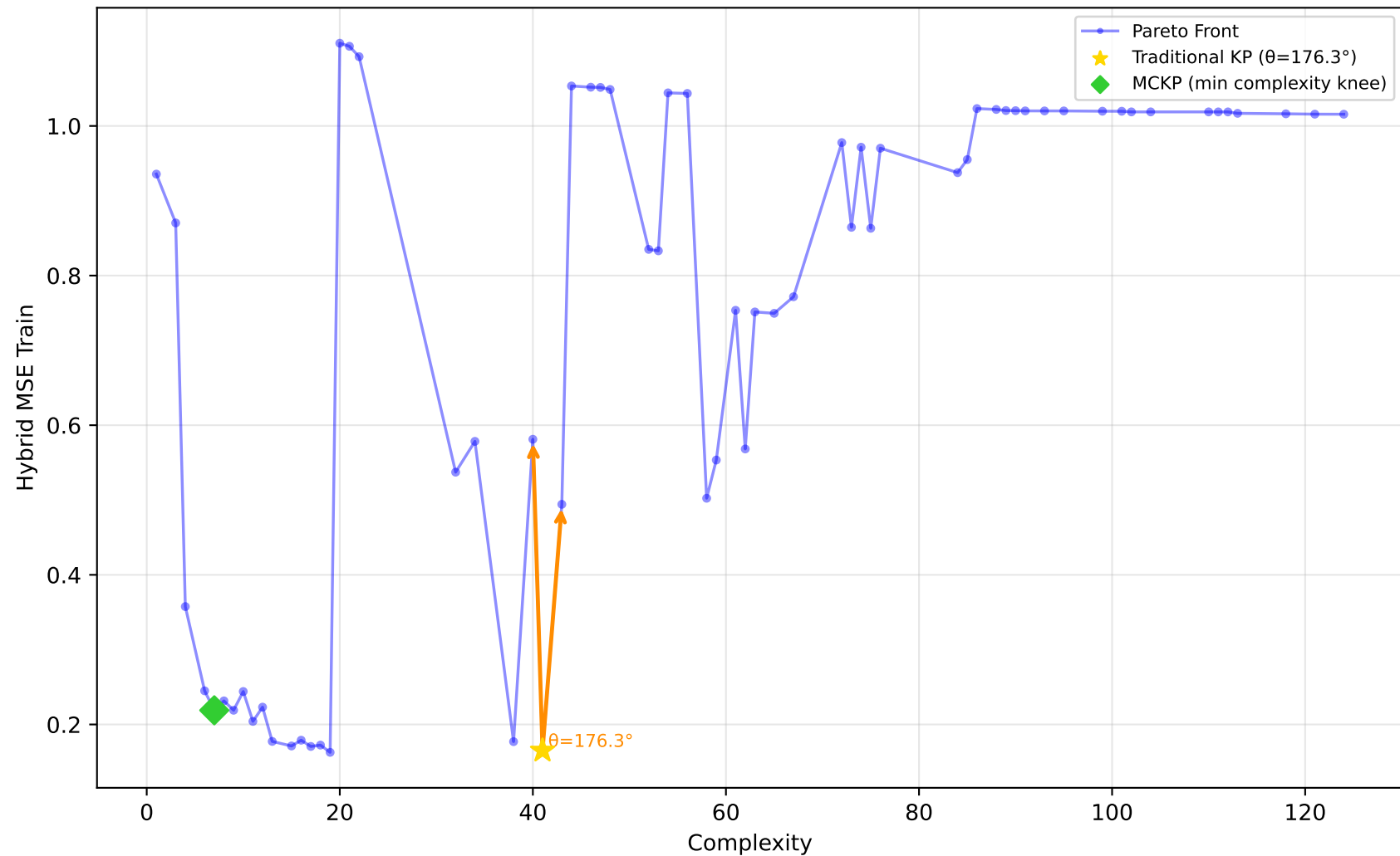
228_elusage - Run 17 - SVP - Hybrid MSE Train \lambda_1=0.00, \bar{\lambda}_2=1.00, \lambda_3=0.00 | Difficulty: 0.69 | Method: hmr
