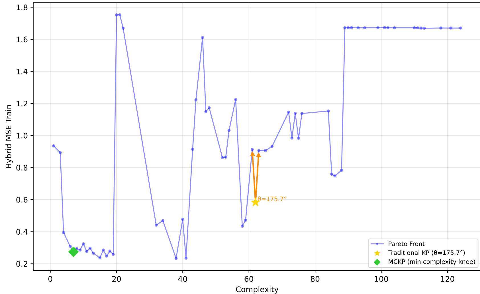
228_elusage - Run 17 - SVP - Hybrid MSE Train \lambda_1=0.60, \bar{\lambda}_2=0.60, \lambda_3=1.00 | Difficulty: 0.69 | Method: hmr
