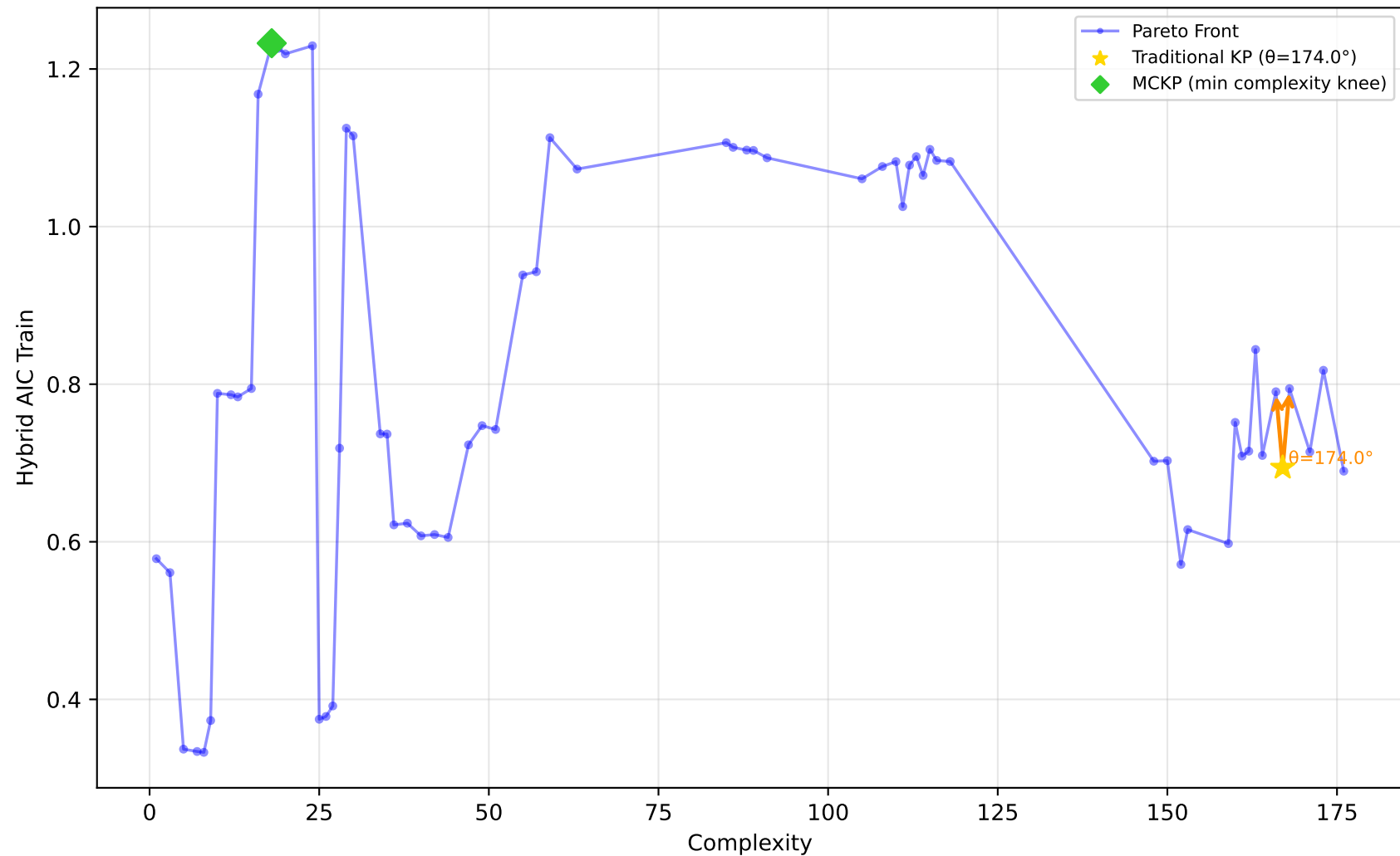
228_elusage - Run 18 - MVP - Hybrid AIC Train \lambda_1=0.00, \bar{\lambda}_2=0.00, \lambda_3=1.00 | Difficulty: 0.77 | Method: hmr
