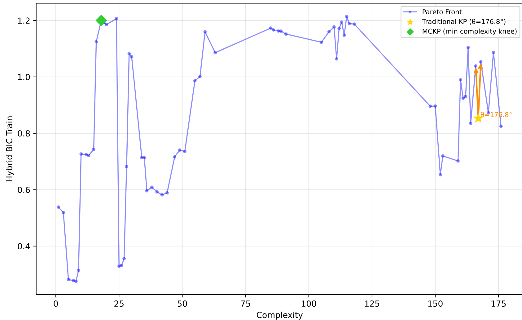
228_elusage - Run 18 - MVP - Hybrid BIC Train \lambda_1=0.00, \bar{\lambda}_2=0.00, \lambda_3=1.00 | Difficulty: 0.77 | Method: hmr
