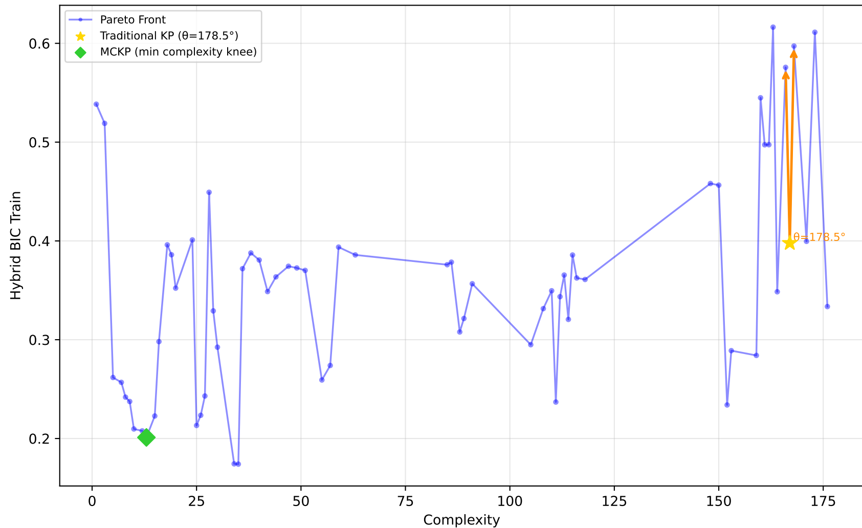
228_elusage - Run 18 - MVP - Hybrid BIC Train \lambda_1=0.00, \lambda_2=0.30, \lambda_3=0.00 | Difficulty: 0.77 | Method: hmr
