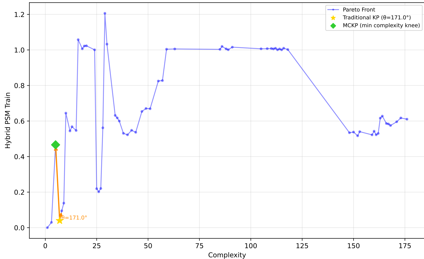
228_elusage - Run 18 - MVP - Hybrid PSM Train \lambda_1=0.00, \bar{\lambda}_2=0.00, \lambda_3=1.00 | Difficulty: 0.77 | Method: hmr
