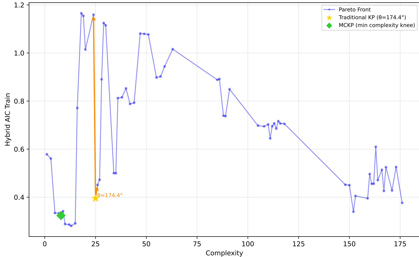
228_elusage - Run 18 - SVP - Hybrid AIC Train \lambda_1=0.00, \lambda_2=1.00, \lambda_3=0.00 | Difficulty: 0.77 | Method: hmr
