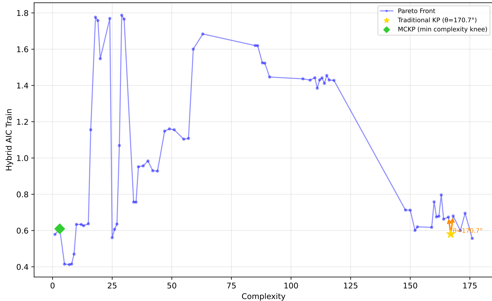
228_elusage - Run 18 - SVP - Hybrid AIC Train \lambda_1=0.60, \lambda_2=0.60, \lambda_3=1.00 | Difficulty: 0.77 | Method: hmr
