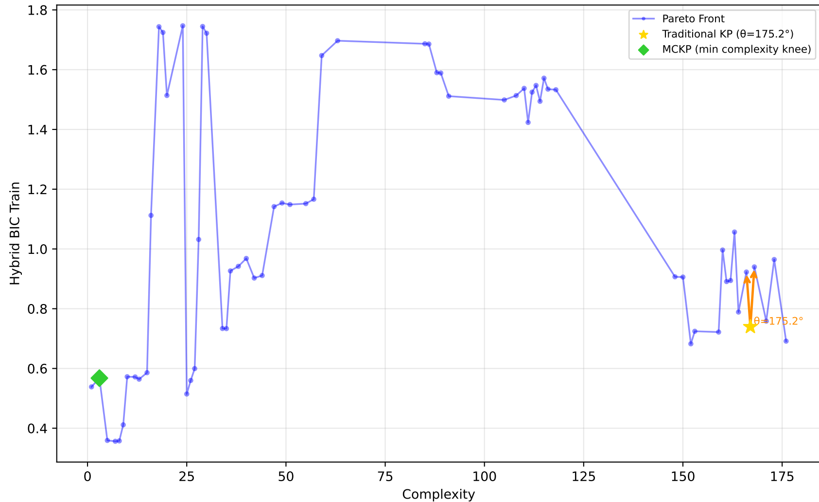
228_elusage - Run 18 - SVP - Hybrid BIC Train \lambda_1=0.60, \lambda_2=0.60, \lambda_3=1.00 | Difficulty: 0.77 | Method: hmr
