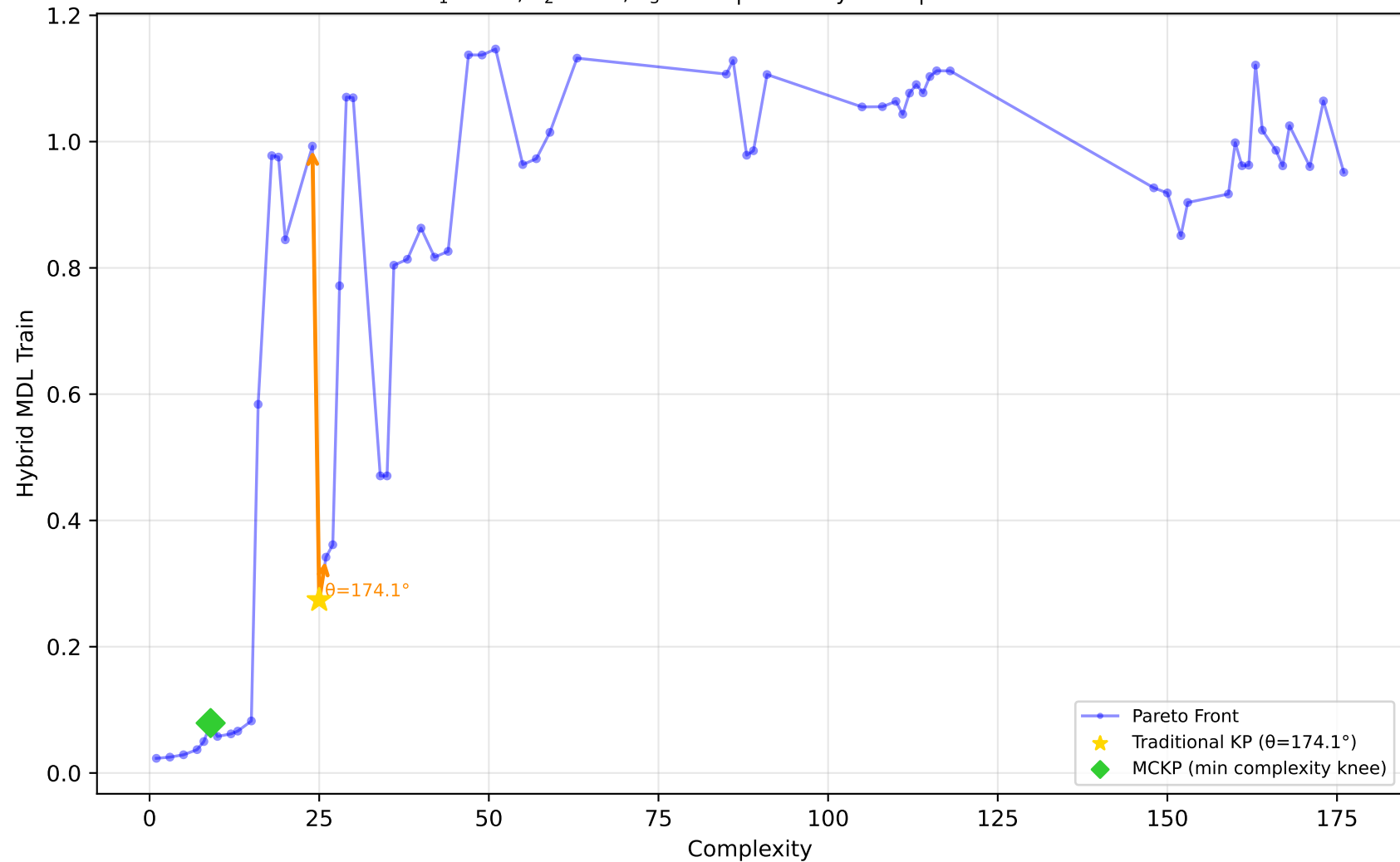
228_elusage - Run 18 - SVP - Hybrid MDL Train \lambda_1=0.00, \bar{\lambda}_2=1.00, \lambda_3=0.00 | Difficulty: 0.77 | Method: hmr
