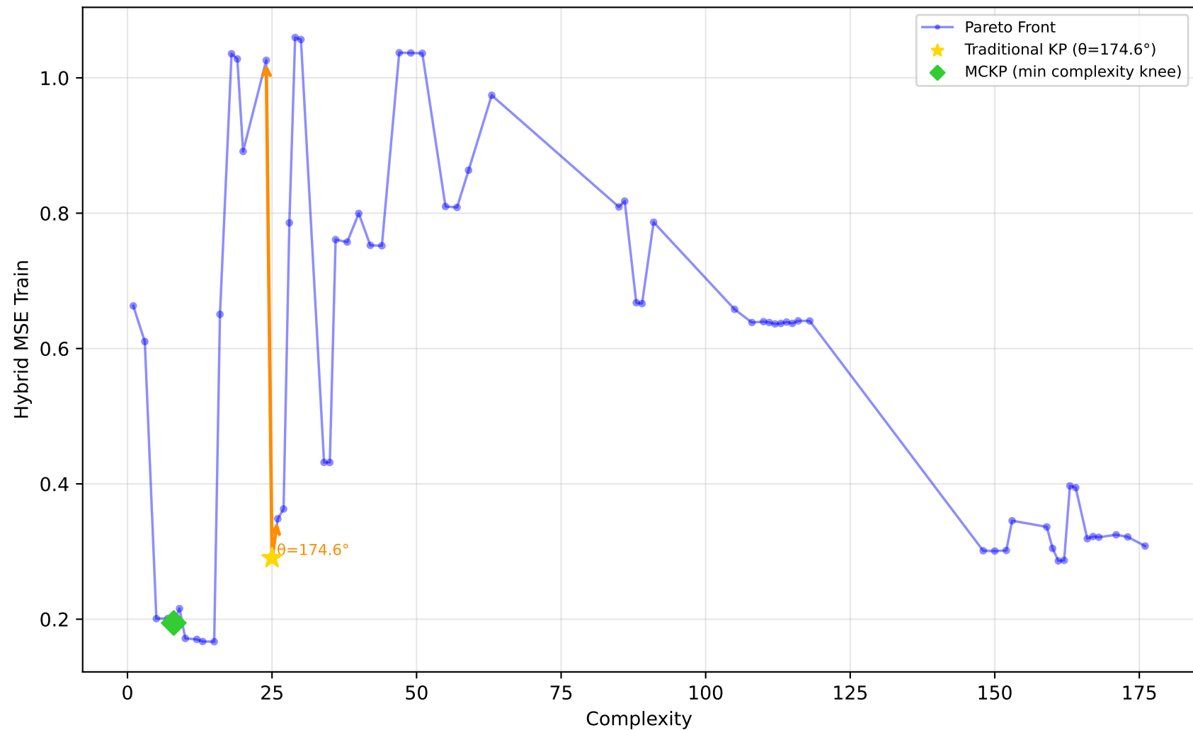
228_elusage - Run 18 - SVP - Hybrid MSE Train \lambda_1=0.00, \bar{\lambda}_2=1.00, \lambda_3=0.00 | Difficulty: 0.77 | Method: hmr
