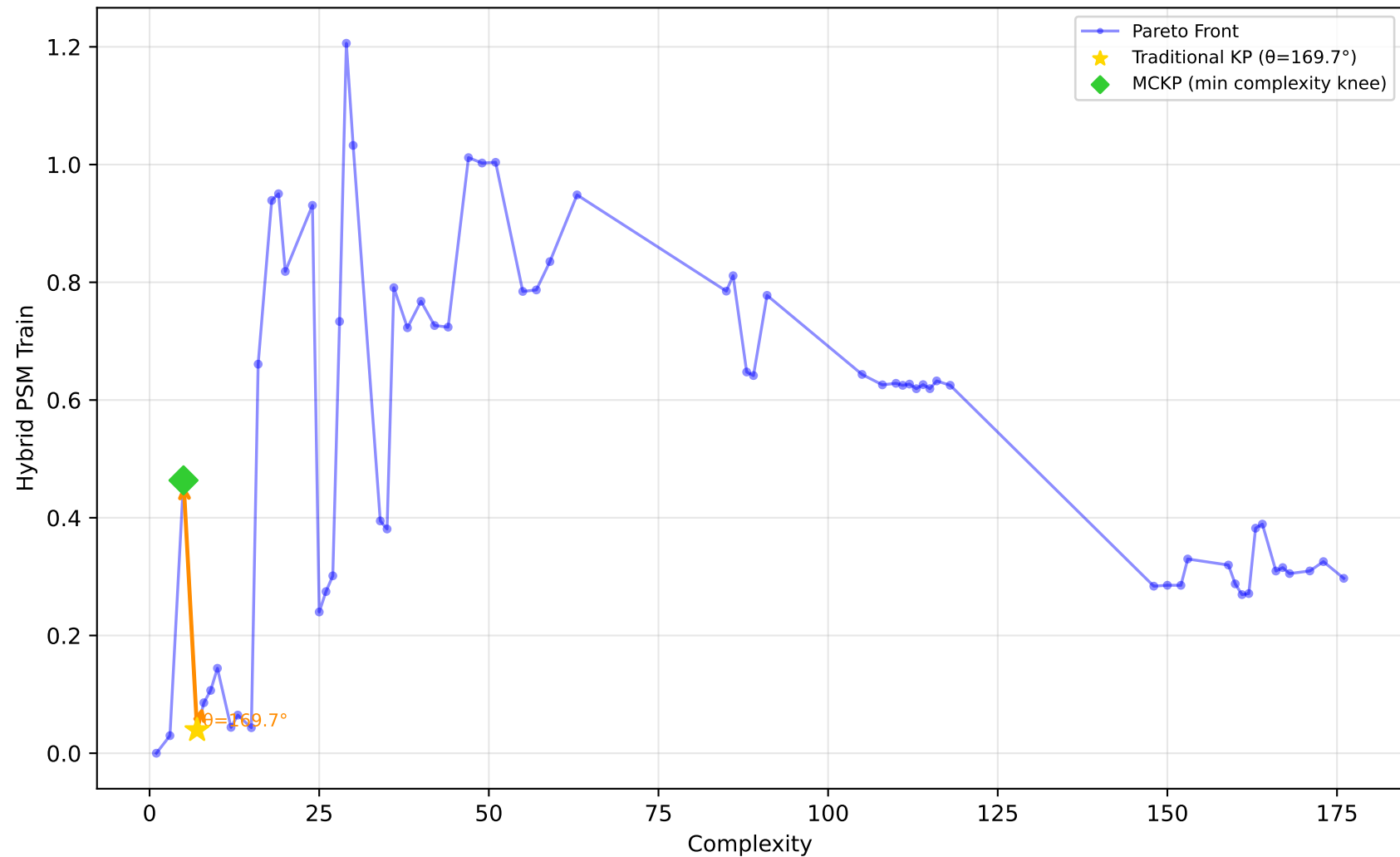
228_elusage - Run 18 - SVP - Hybrid PSM Train \lambda_1=0.00, \bar{\lambda}_2=1.00, \lambda_3=0.00 | Difficulty: 0.77 | Method: hmr
