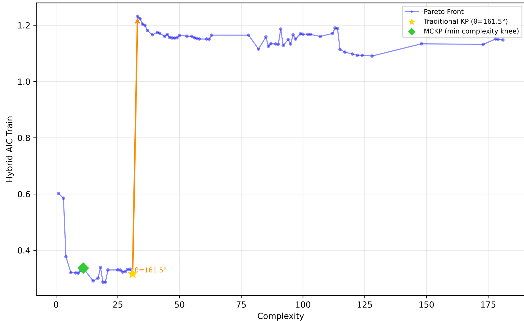
228_elusage - Run 19 - MVP - Hybrid AIC Train \lambda_1=0.00, \lambda_2=0.00, \lambda_3=1.00 | Difficulty: 1.00 | Method: hmr
