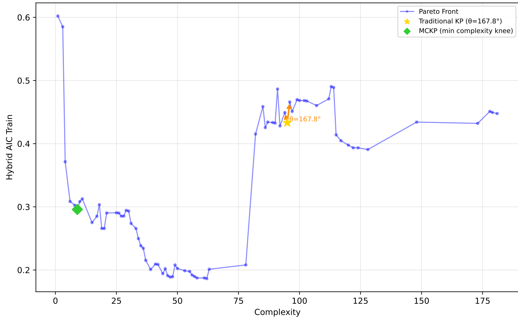
228_elusage - Run 19 - MVP - Hybrid AIC Train \lambda_1=0.00, \lambda_2=0.30, \lambda_3=0.00 | Difficulty: 1.00 | Method: hmr
