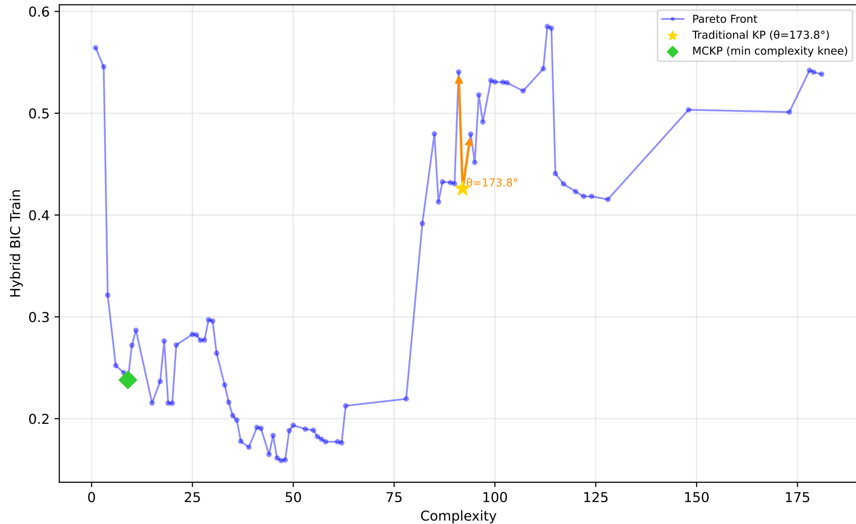
228_elusage - Run 19 - MVP - Hybrid BIC Train \lambda_1=0.00, \lambda_2=0.30, \lambda_3=0.00 | Difficulty: 1.00 | Method: hmr
