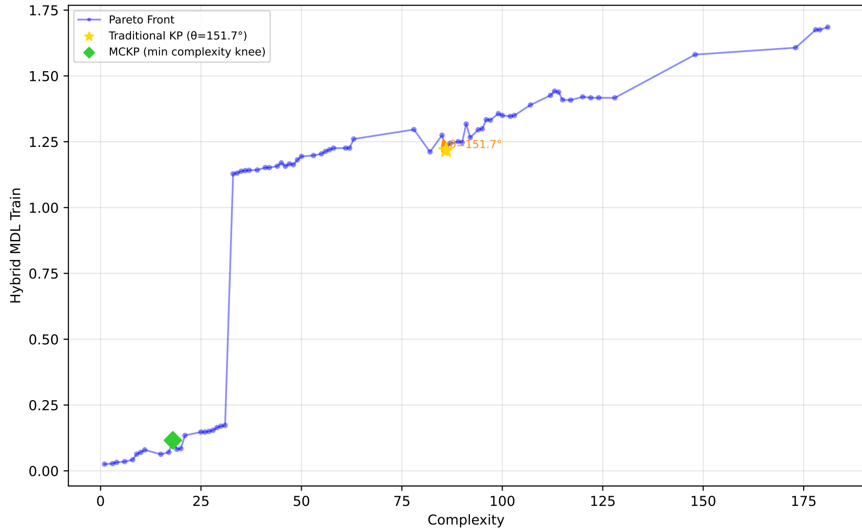
228_elusage - Run 19 - MVP - Hybrid MDL Train \lambda_1=0.00, \bar{\lambda}_2=0.00, \lambda_3=1.00 | Difficulty: 1.00 | Method: hmr
