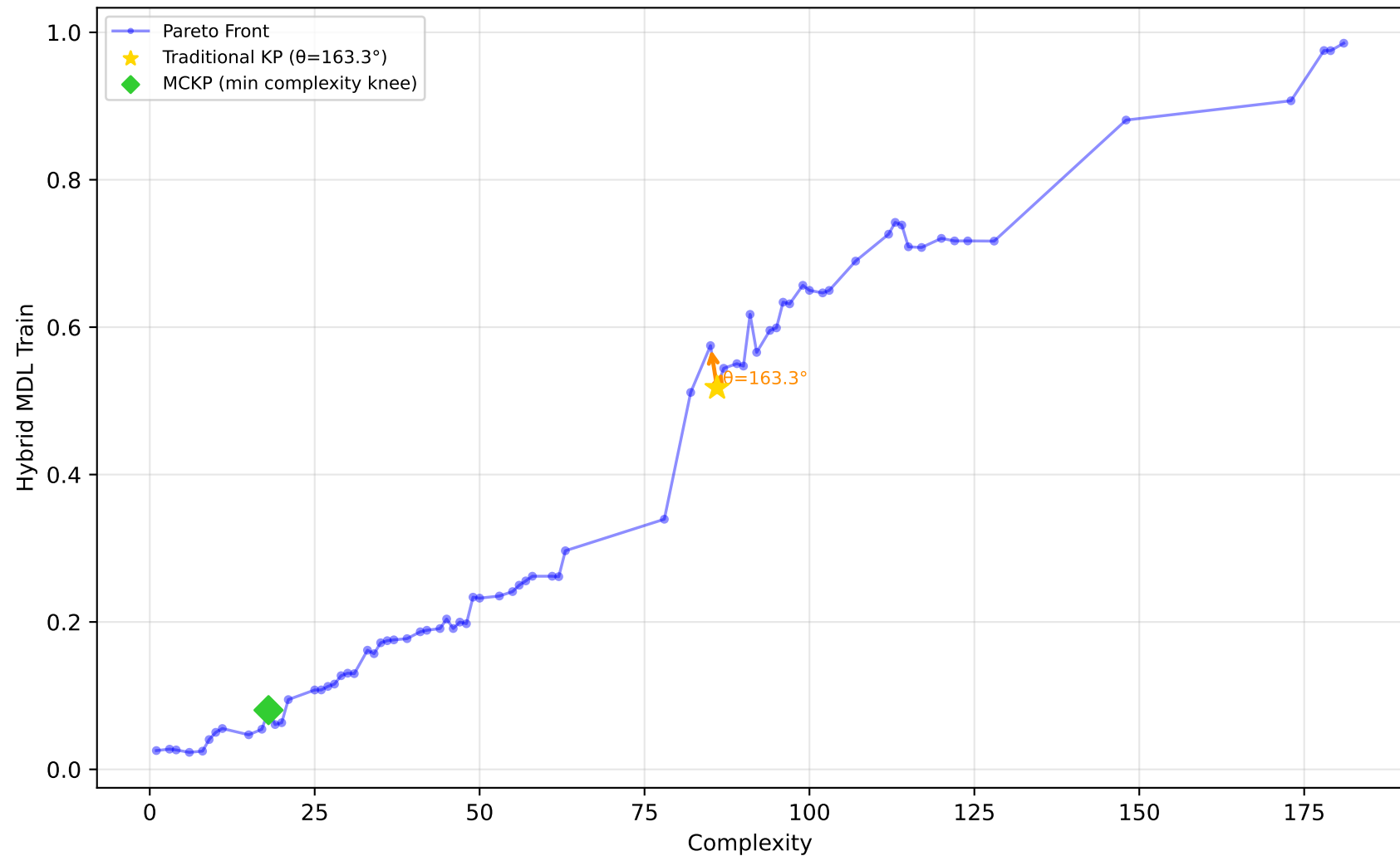
228_elusage - Run 19 - MVP - Hybrid MDL Train \lambda_1=0.00, \bar{\lambda}_2=0.30, \lambda_3=0.00 | Difficulty: 1.00 | Method: hmr
