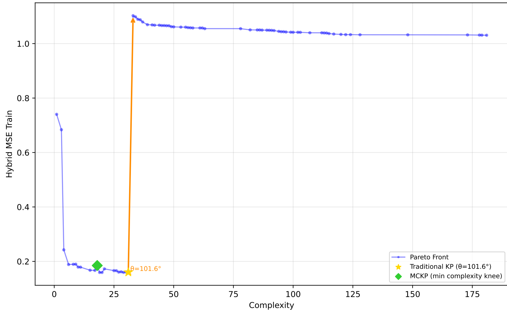
228_elusage - Run 19 - MVP - Hybrid MSE Train \lambda_1=0.00, \bar{\lambda}_2=0.00, \lambda_3=1.00 | Difficulty: 1.00 | Method: hmr
