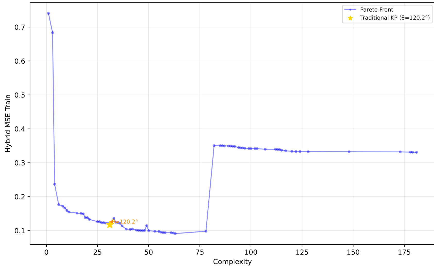
228_elusage - Run 19 - MVP - Hybrid MSE Train \lambda_1=0.00, \bar{\lambda}_2=0.30, \lambda_3=0.00 | Difficulty: 1.00 | Method: hmr
