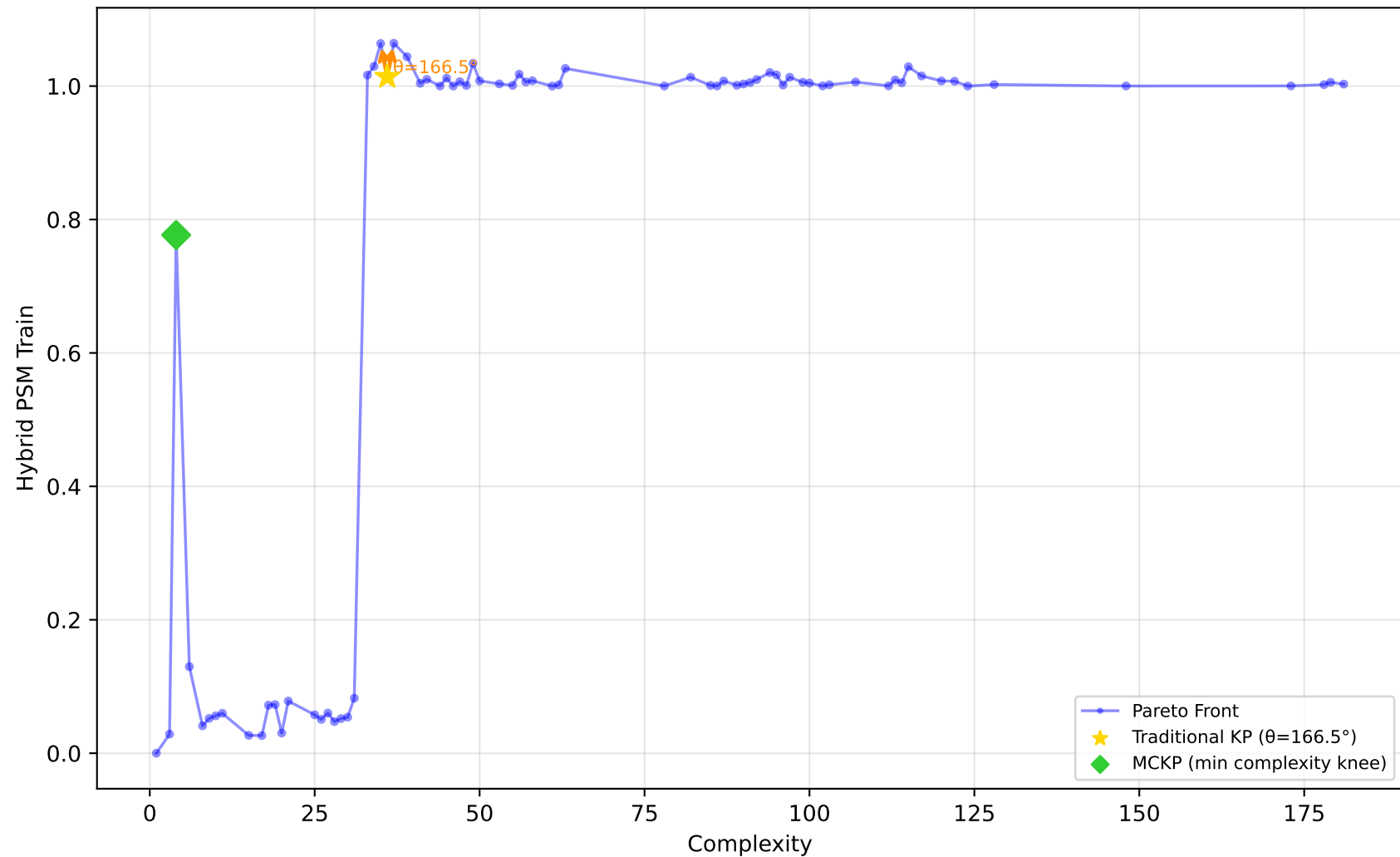
228_elusage - Run 19 - MVP - Hybrid PSM Train \lambda_1=0.00, \bar{\lambda}_2=0.00, \lambda_3=1.00 | Difficulty: 1.00 | Method: hmr
