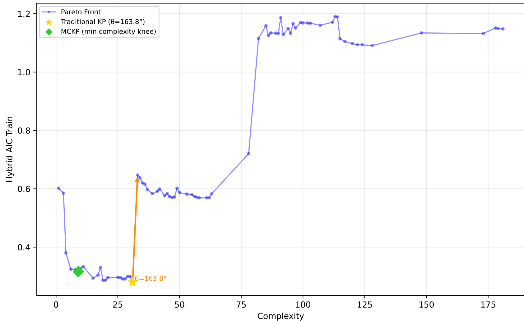
228_elusage - Run 19 - SVP - Hybrid AIC Train \lambda_1=0.00, \lambda_2=1.00, \lambda_3=0.00 | Difficulty: 1.00 | Method: hmr
