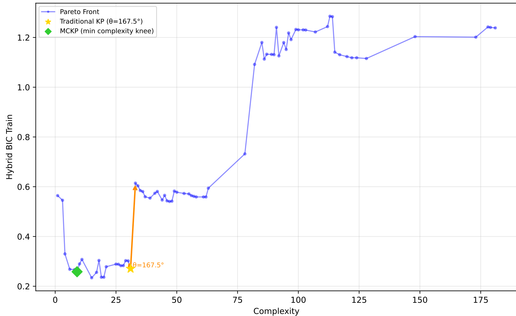
228_elusage - Run 19 - SVP - Hybrid BIC Train \lambda_1=0.00, \lambda_2=1.00, \lambda_3=0.00 | Difficulty: 1.00 | Method: hmr
