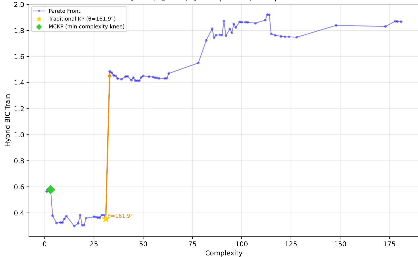
228_elusage - Run 19 - SVP - Hybrid BIC Train \lambda_1=0.60, \lambda_2=0.60, \lambda_3=1.00 | Difficulty: 1.00 | Method: hmr
