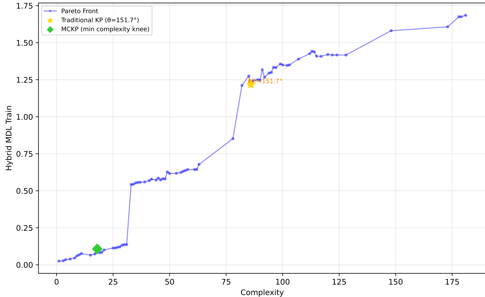
228_elusage - Run 19 - SVP - Hybrid MDL Train \lambda_1=0.00 , \bar{\lambda}_2=1.00 , \lambda_3=0.00 | Difficulty: 1.00 | Method: hmr
