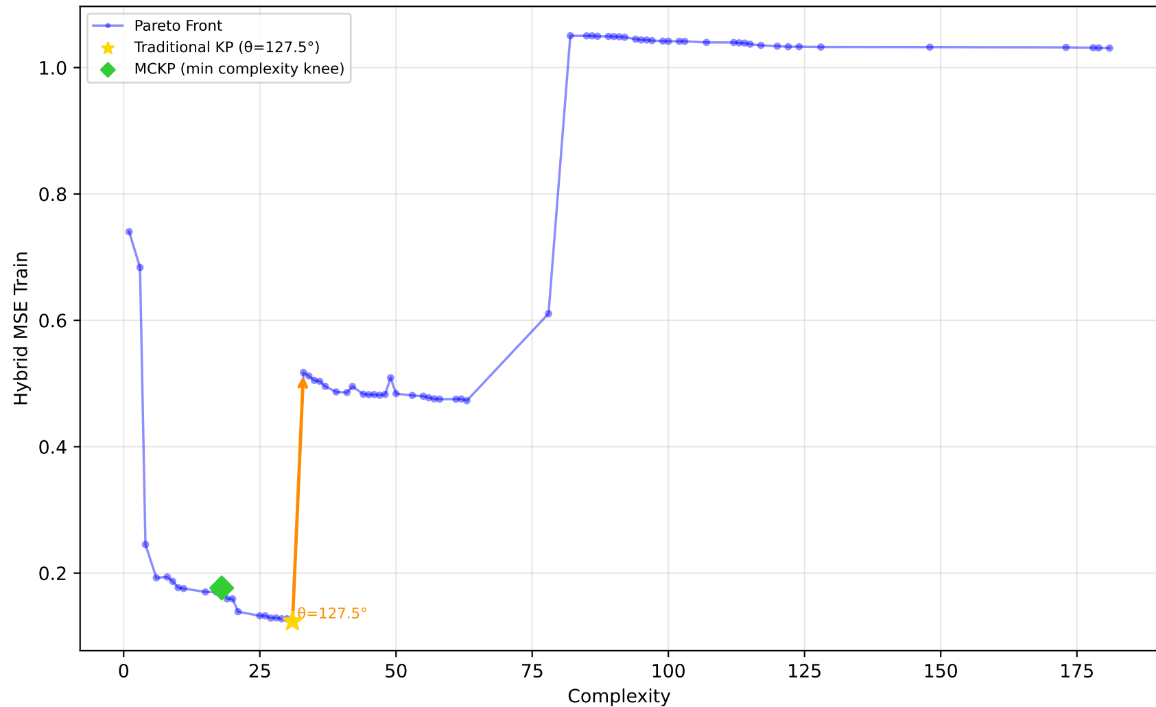
228_elusage - Run 19 - SVP - Hybrid MSE Train \lambda_1=0.00, \bar{\lambda}_2=1.00, \lambda_3=0.00 | Difficulty: 1.00 | Method: hmr
