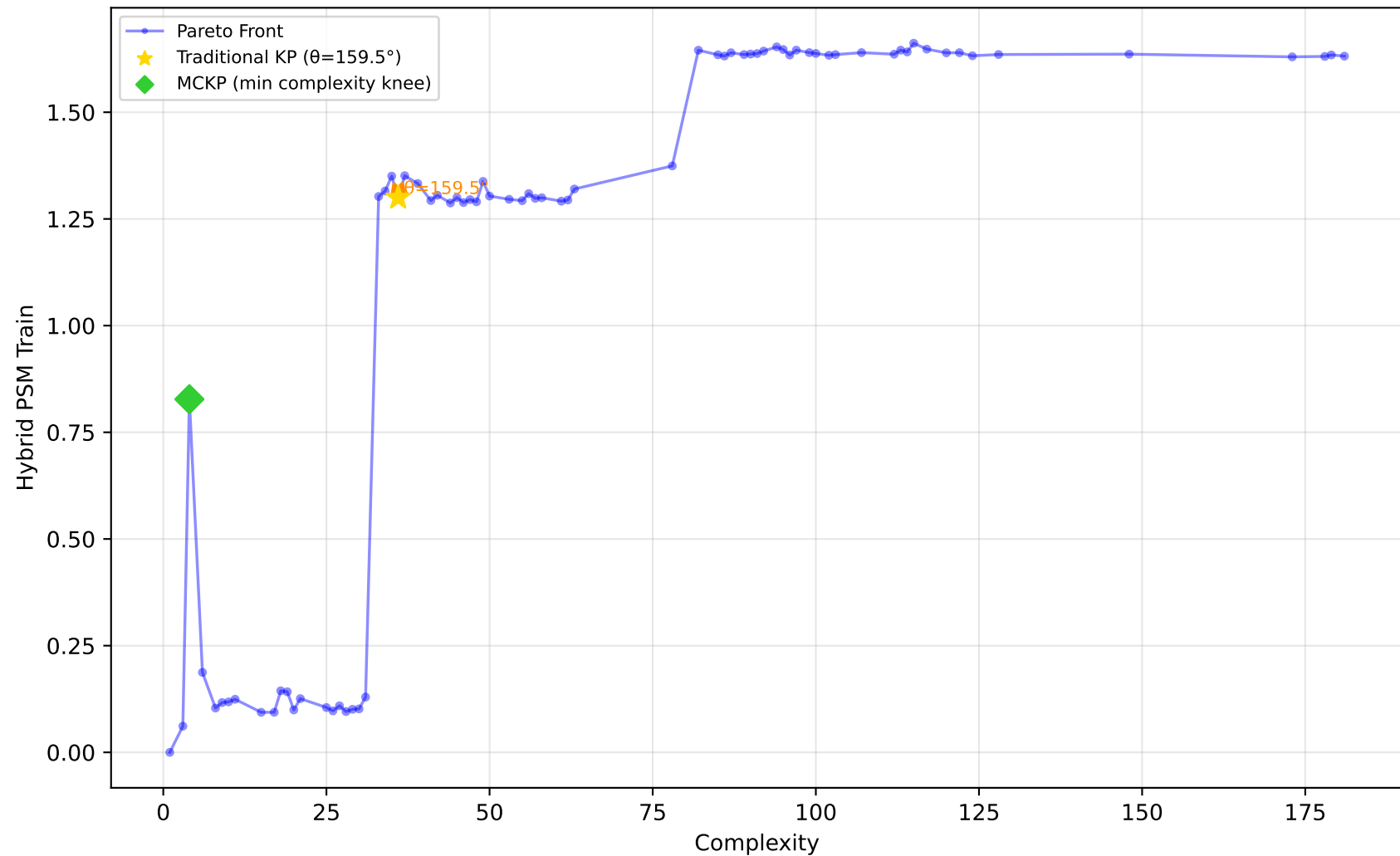
228_elusage - Run 19 - SVP - Hybrid PSM Train \lambda_1=0.60, \bar{\lambda}_2=0.60, \lambda_3=1.00 | Difficulty: 1.00 | Method: hmr
