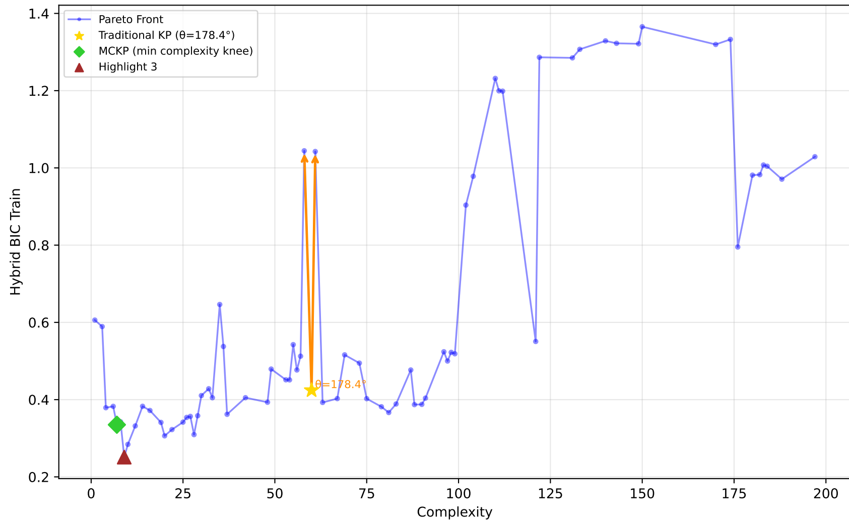
228_elusage - Run 1 - MVP - Hybrid BIC Train \lambda_1=0.00, \lambda_2=0.00, \lambda_3=1.00 | Difficulty: 0.83 | Method: hmr
