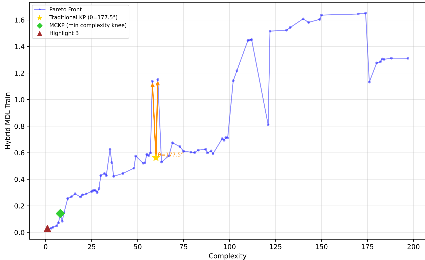
228_elusage - Run 1 - MVP - Hybrid MDL Train \lambda_1=0.00, \lambda_2=0.00, \lambda_3=1.00 | Difficulty: 0.83 | Method: hmr
