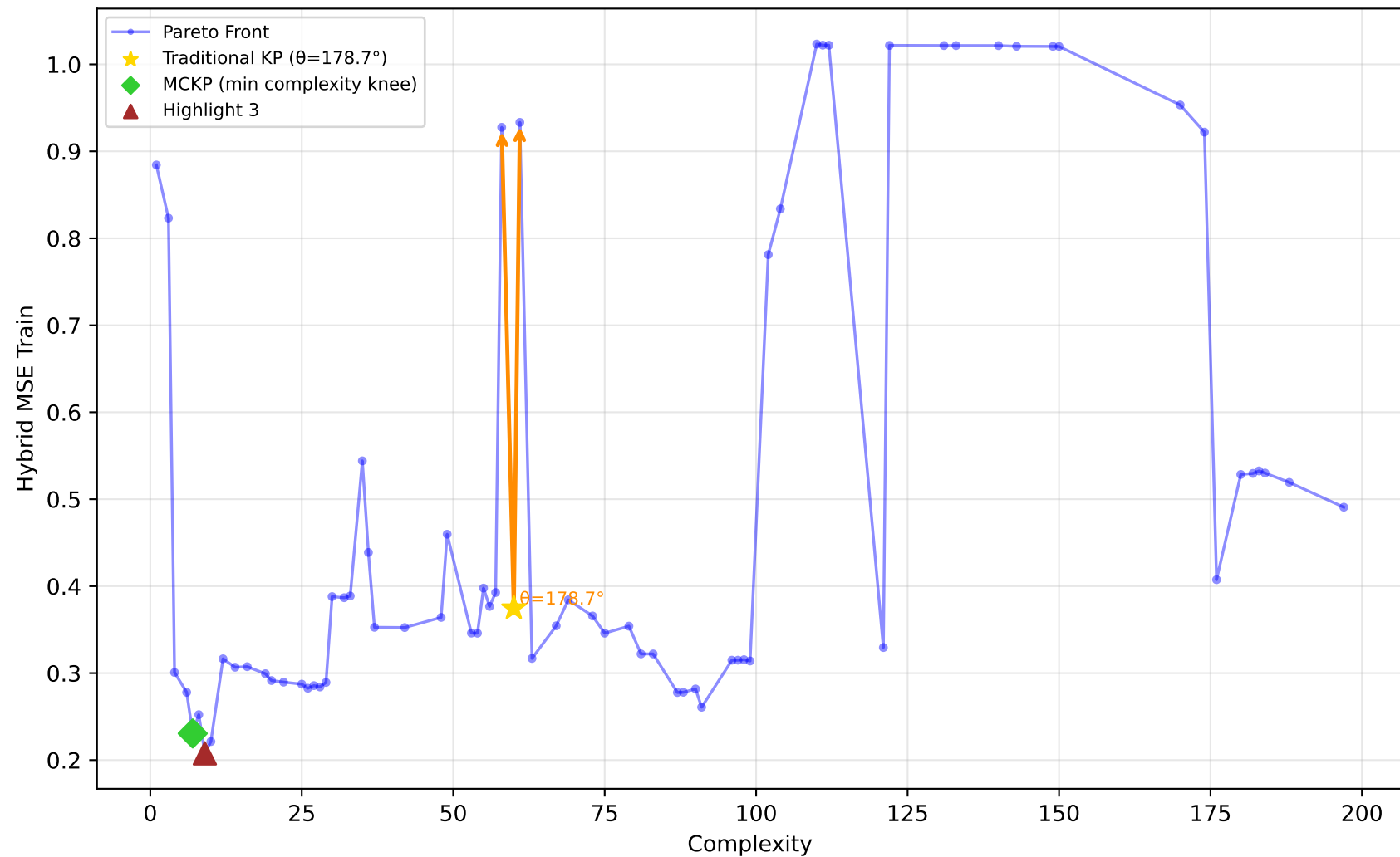
228_elusage - Run 1 - MVP - Hybrid MSE Train \lambda_1=0.00, \lambda_2=0.00, \lambda_3=1.00 | Difficulty: 0.83 | Method: hmr
