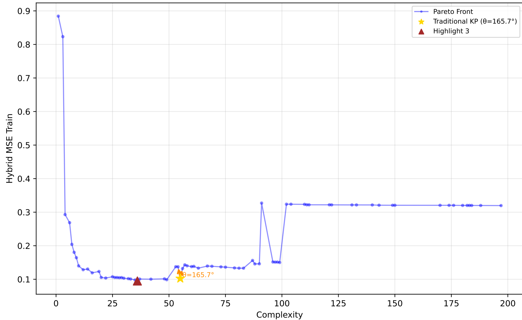
228_elusage - Run 1 - MVP - Hybrid MSE Train \lambda_1=0.00, \lambda_2=0.30, \lambda_3=0.00 | Difficulty: 0.83 | Method: hmr
