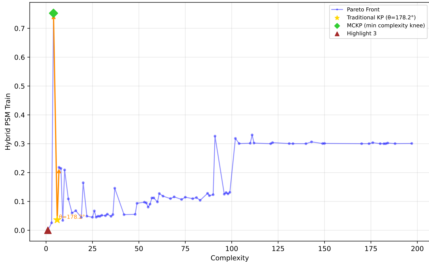
228_elusage - Run 1 - MVP - Hybrid PSM Train \lambda_1=0.00, \lambda_2=0.30, \lambda_3=0.00 | Difficulty: 0.83 | Method: hmr
