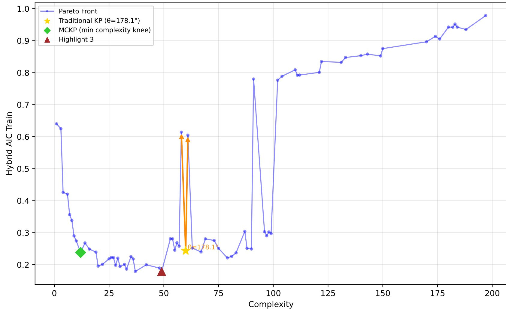
228_elusage - Run 1 - SVP - Hybrid AIC Train \lambda_1=0.00, \lambda_2=1.00, \lambda_3=0.00 | Difficulty: 0.83 | Method: hmr
