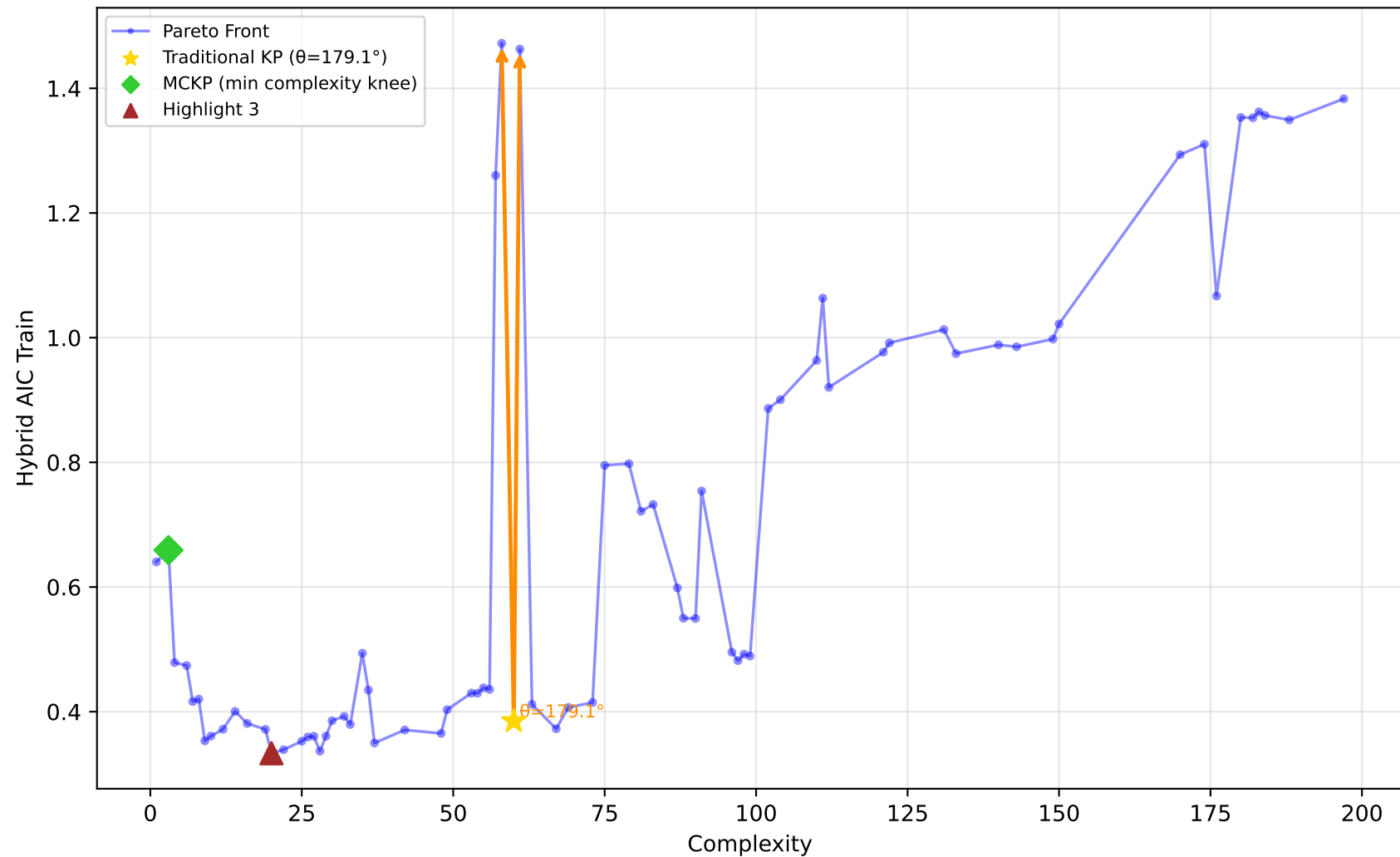
228_elusage - Run 1 - SVP - Hybrid AIC Train \lambda_1=0.60, \lambda_2=0.60, \lambda_3=1.00 | Difficulty: 0.83 | Method: hmr
