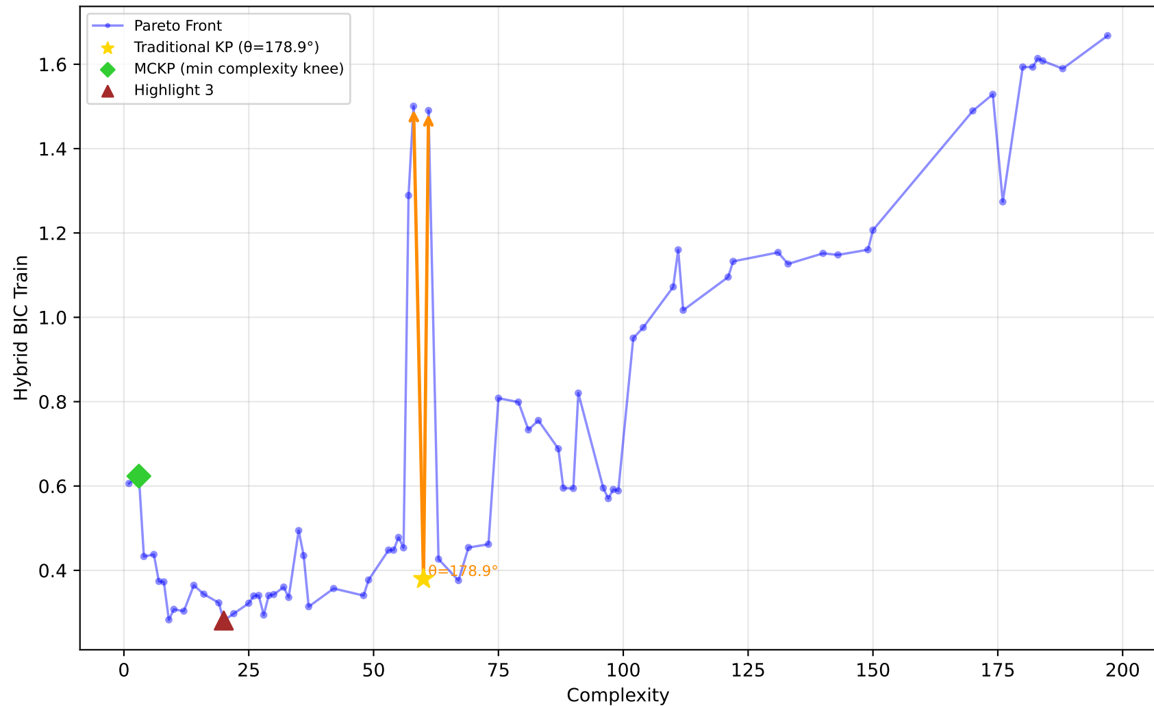
228_elusage - Run 1 - SVP - Hybrid BIC Train \lambda_1=0.60, \lambda_2=0.60, \lambda_3=1.00 | Difficulty: 0.83 | Method: hmr
