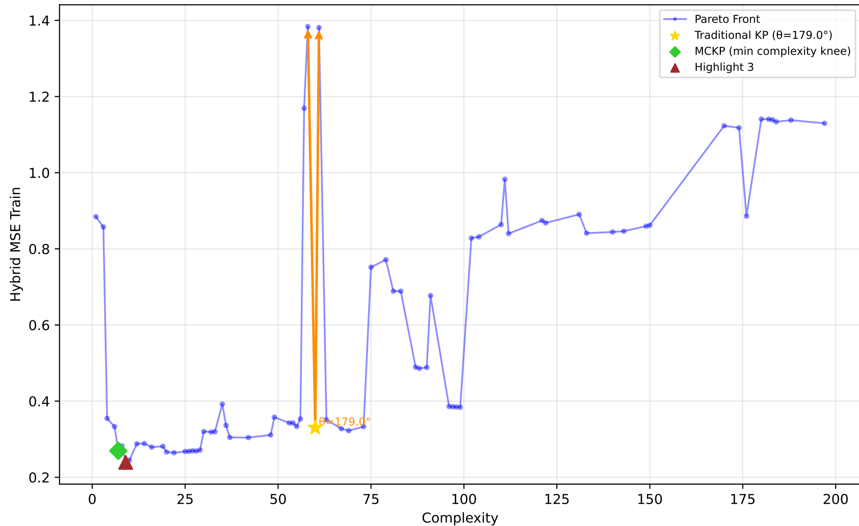
228_elusage - Run 1 - SVP - Hybrid MSE Train \lambda_1=0.60, \lambda_2=0.60, \lambda_3=1.00 | Difficulty: 0.83 | Method: hmr
