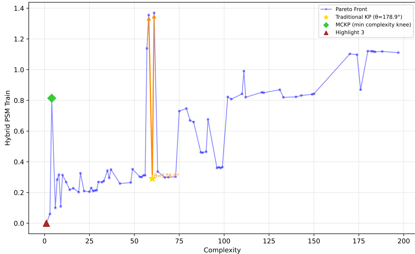
228_elusage - Run 1 - SVP - Hybrid PSM Train \lambda_1=0.60, \lambda_2=0.60, \lambda_3=1.00 | Difficulty: 0.83 | Method: hmr
